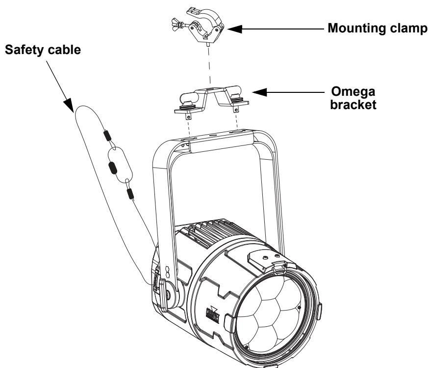
Overhead mounting
