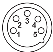
DMX-stekker
