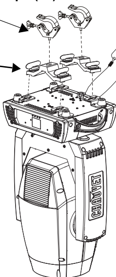
Overhead Mounting
