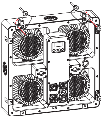
Latch button
