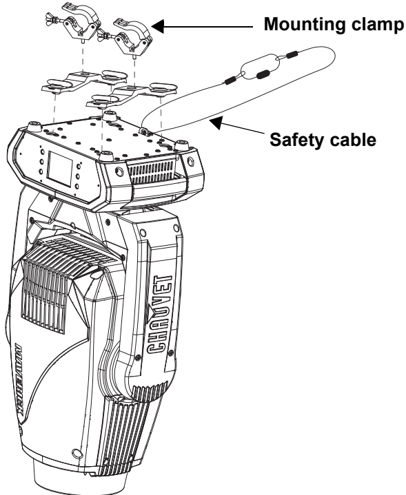
Overhead Mounting
